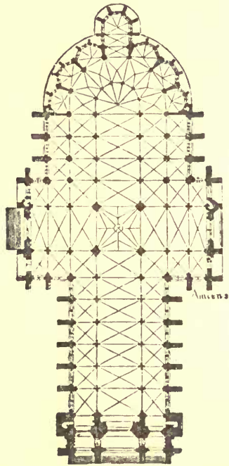
GROUND-PLAN OF THE CATHEDRAL OF AMIENS
